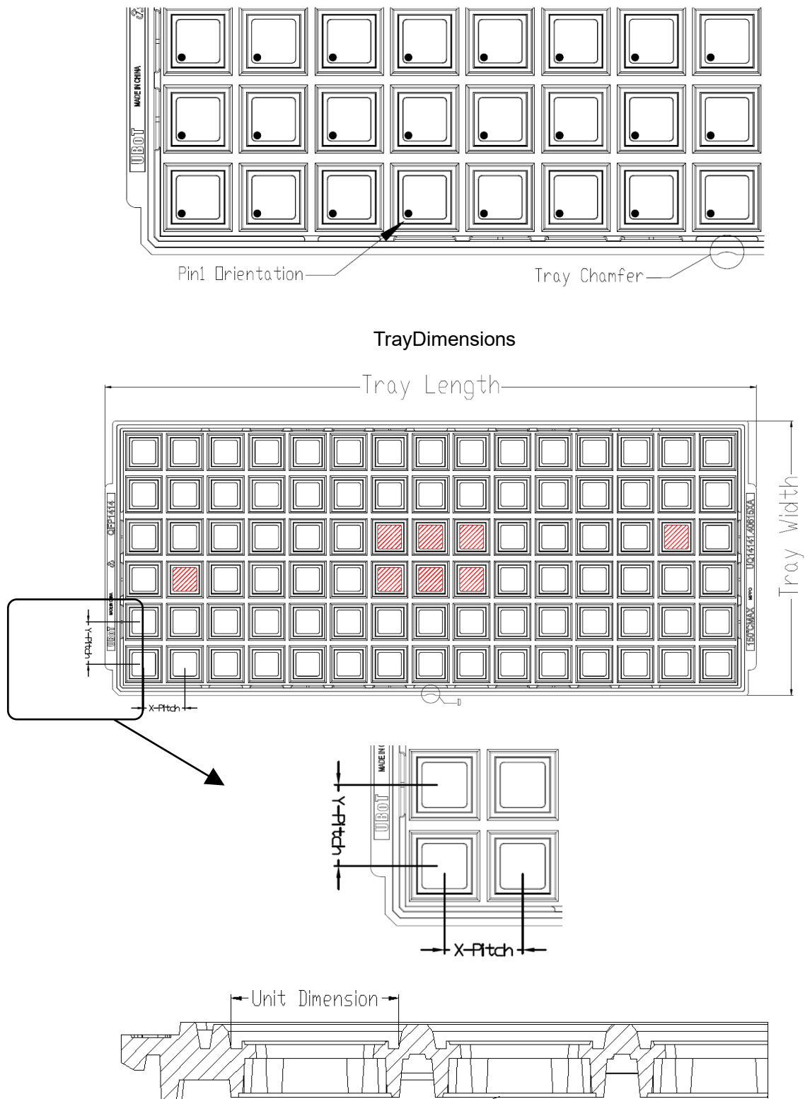
Figure 26 Tray Packaging Schematic Diagram
