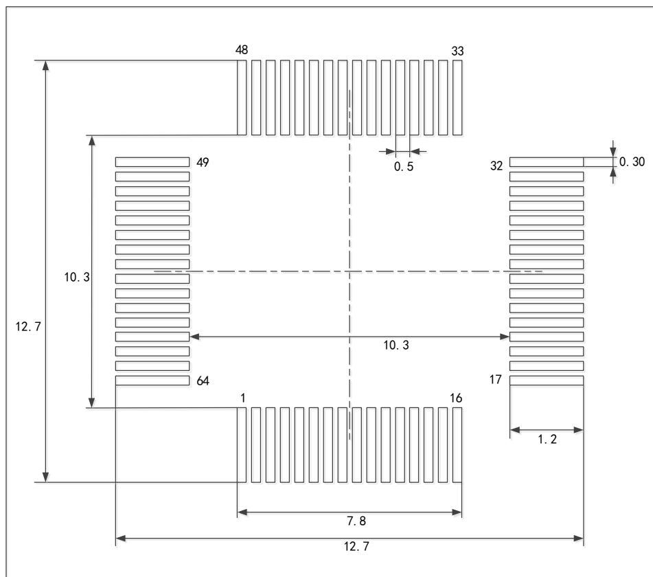
Figure 19 LQFP64 Welding Layout Suggestion
