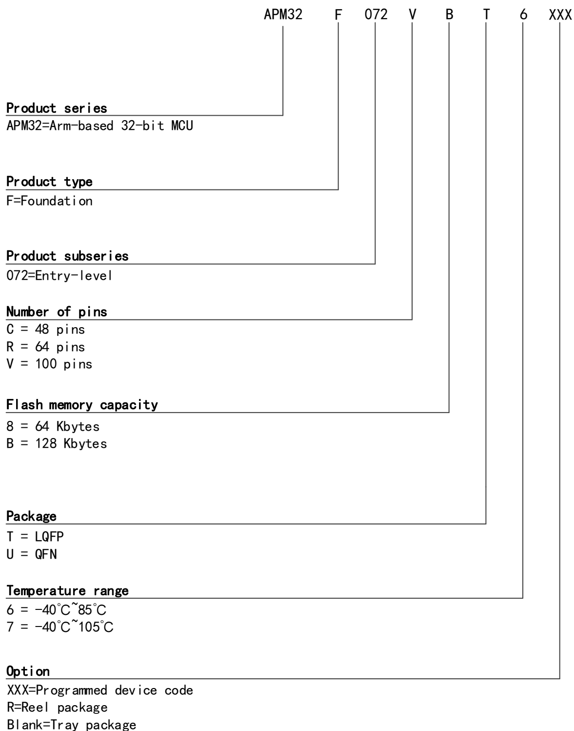
Figure 27 Naming Rules of Ordering Information
