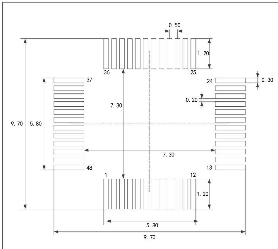
Figure 21 LQFP48 Welding Layout Suggestion
