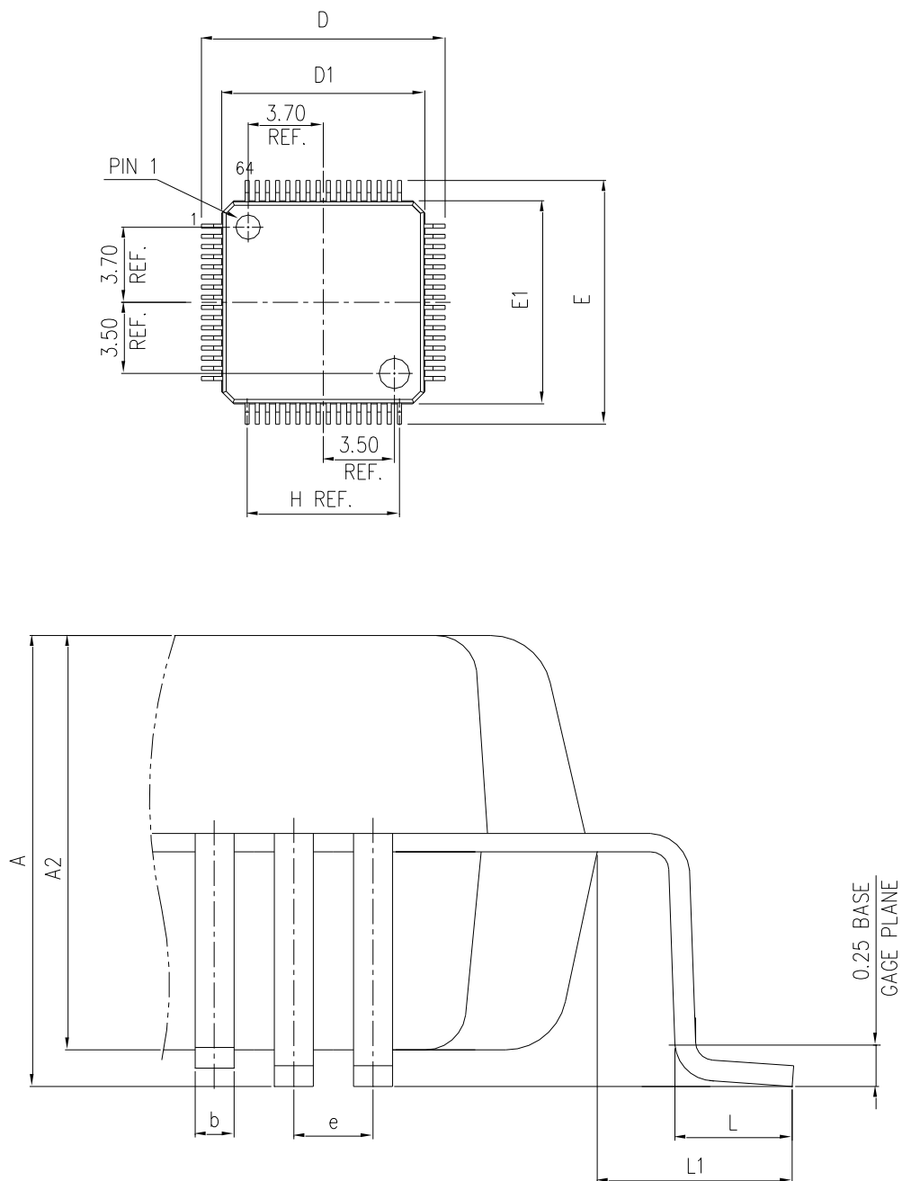
Figure 18 LQFP64 Package Diagram
