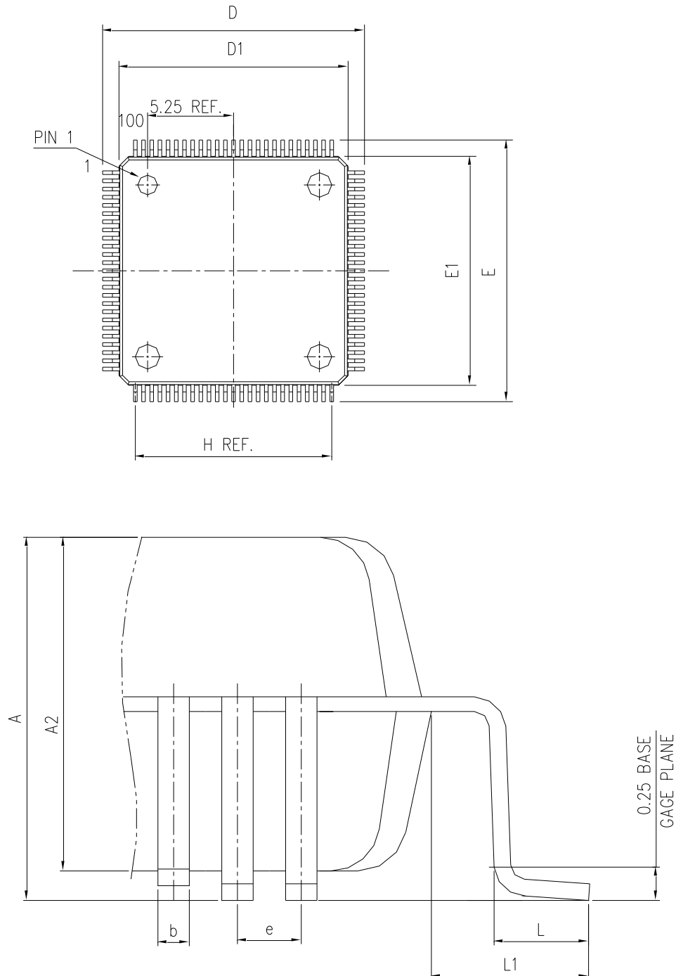
Figure 16 Package Diagram of LQFP100
