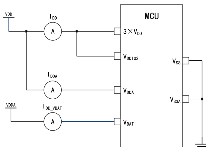
Figure 10 Power Consumption Measurement Scheme
