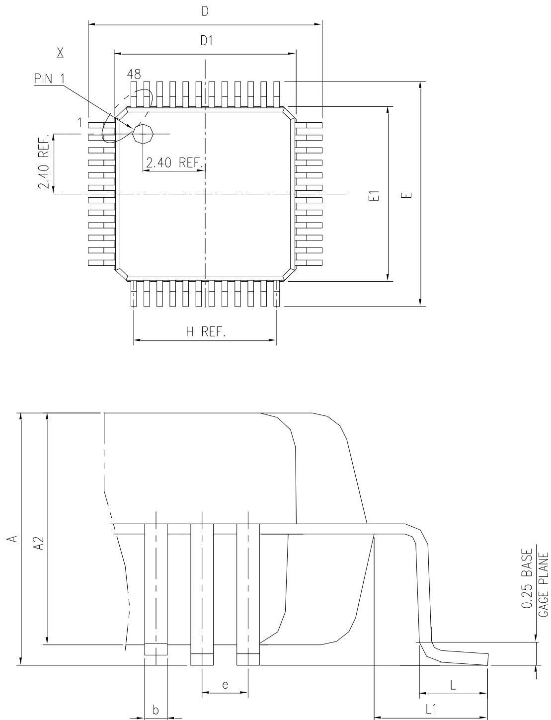
Figure 20 LQFP48 Package Diagram
